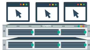
Server virtualization
